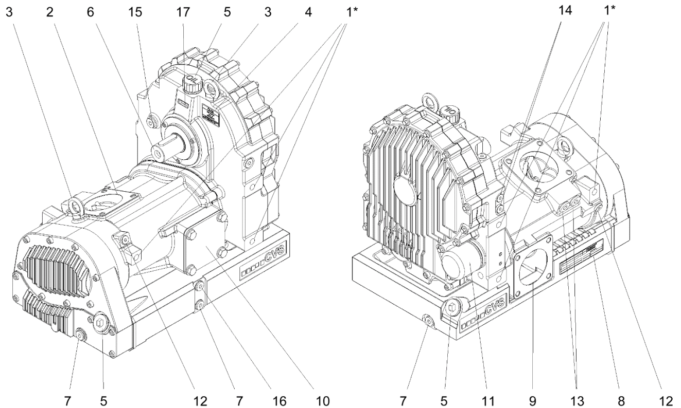
Fig. 1: Compressor view
