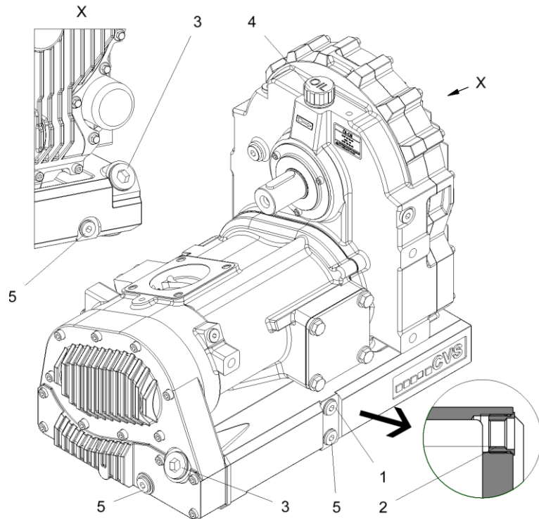
Fig. 4: Oil level and oil change
